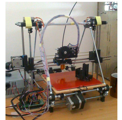
RepRap Prusa
