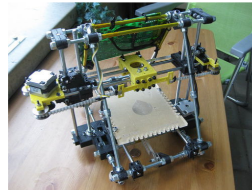
RepRap Huxley
